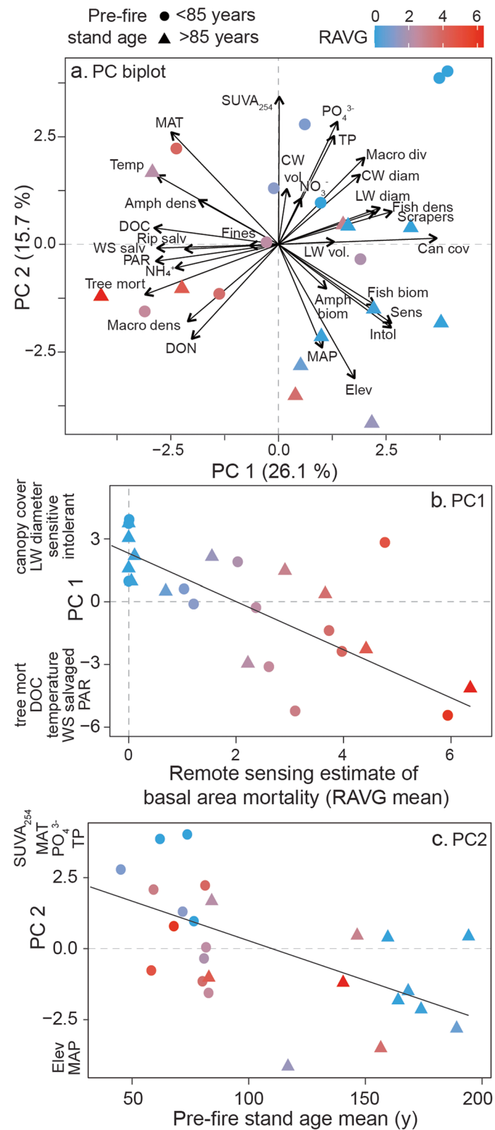
Fig. 5 Principal components analysis (PCA) and relationships of axes with fire severity and pre-fire stand age. a PCA with scores and loadings of physical, chemical, biological, and watershed characteristics. b Principal component 1 (PC1) varied as a function of fire severity as RAVG mean. c Principal component 2 (PC2) varied as a function of pre-fire stand age
